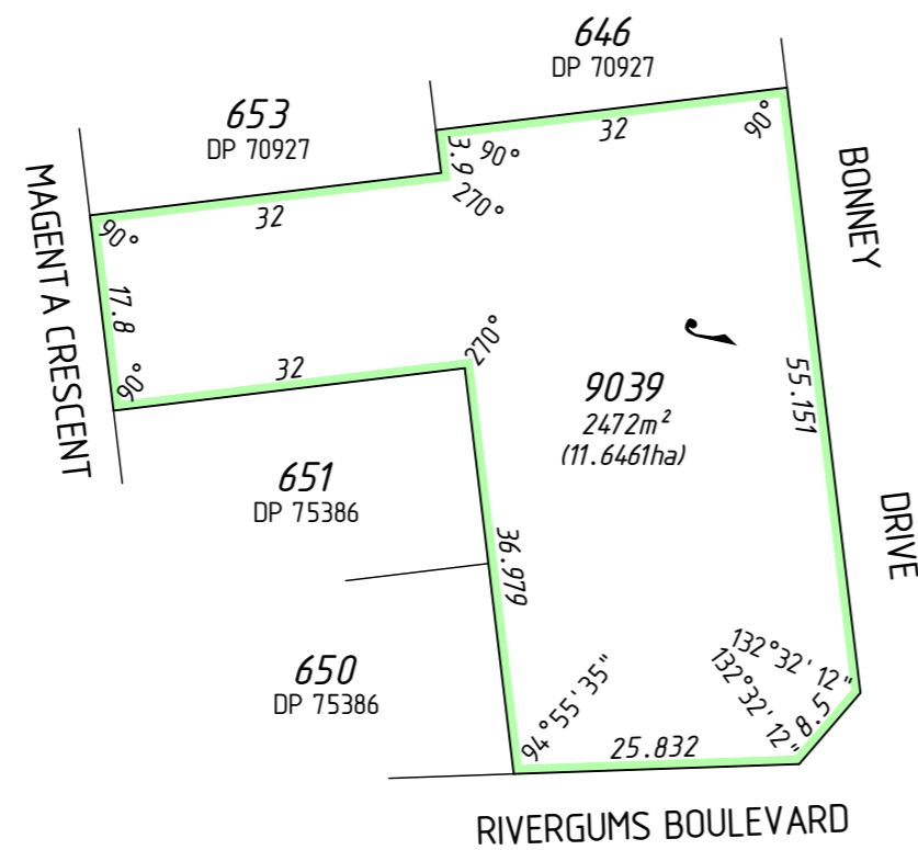
ENLARGEMENT 'A1' Not to scale
